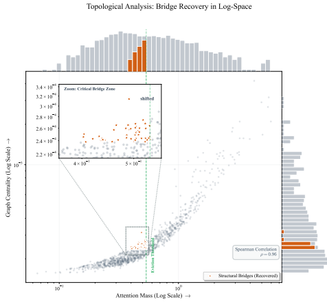
Figure 4: Centrality vs. Attention (Log-Space) . Tokens with low direct attention but high graph centrality (Orange Stars) are identified as “Structural Bridges.” Masking them reduces reasoning performance. (Plot generated via automated analysis of Llama-3 attention maps).
