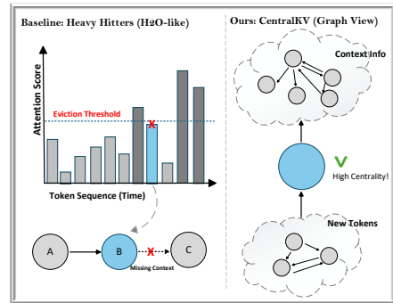
Figure 1: Conceptual Comparison. (Left) Heavy-hitter methods (e.g., H2O) discard critical “Structural Bridges” (blue) with low local attention. (Right) CentralKV identifies these bridges via graph centrality, preserving the reasoning chain.
