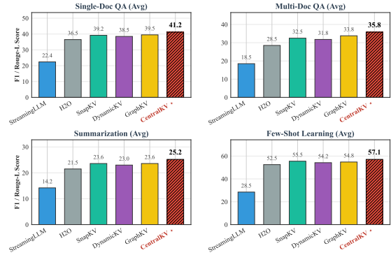
Figure 5: Performance by Task Category. On the four categories shown (Single-Doc QA, Multi-Doc QA, Summarization, Few-Shot Learning), CentralKV (red striped) achieves the highest scores, consistently outperforming GraphKV in Multi-Doc QA and Few-Shot tasks.
