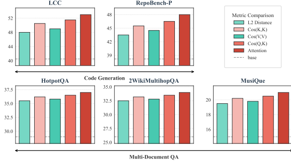
Figure 6: Metric Ablation. Attention-based graph construction (Red) consistently outperforms L2 and Cosine similarity metrics, particularly in Multi-Doc QA.
