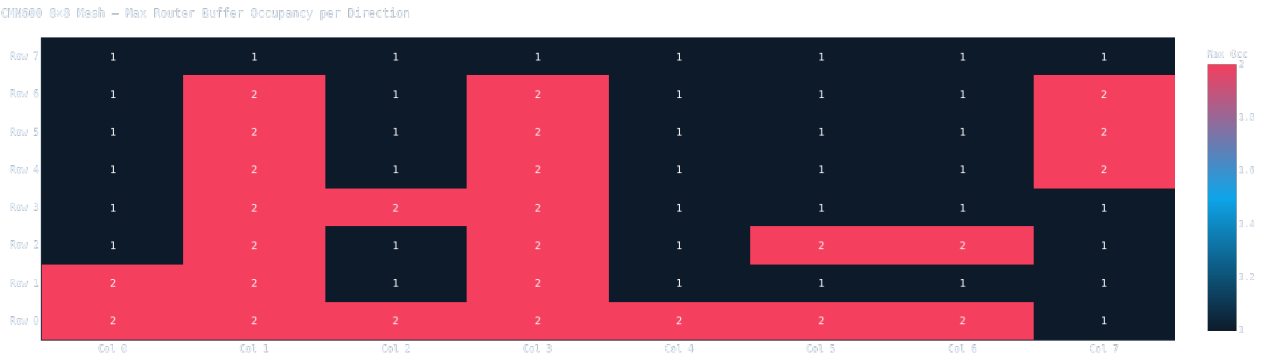
Figure 12: CMN600 8x8 Mesh Router Buffer Occupancy Heatmap (Cache & Memory tab)
