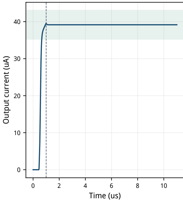
1 us supply ramp
