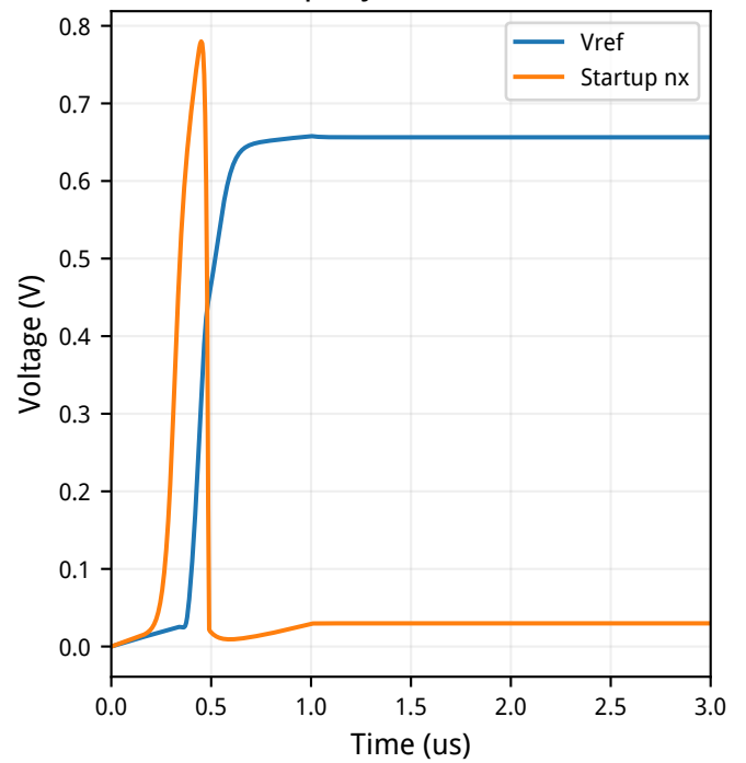
Startup injection turns off
