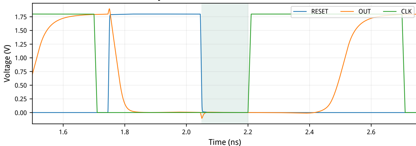
Asynchronous assertion and release
