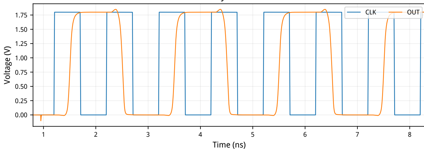
Divide by 2 at 1 GHz
