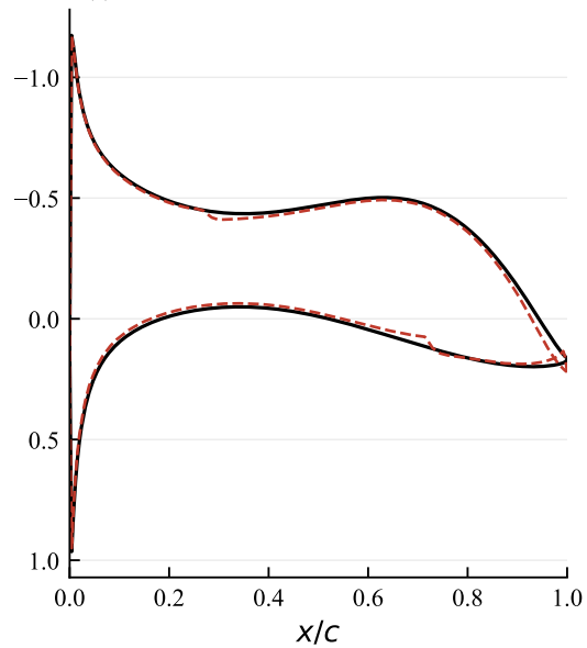
(a) M = 0.30 , \alpha = 2.1^\circ , Re = 1.7 \times 10^6
