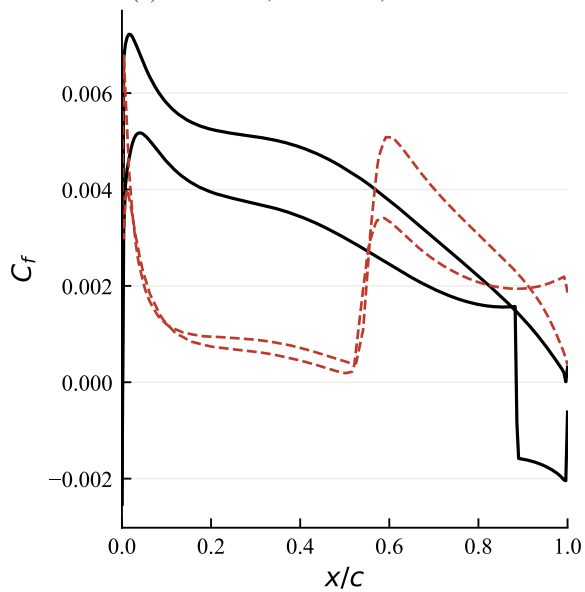
(b) M = 0.50 , \alpha = 1.1^\circ , Re = 5.1 \times 10^6
