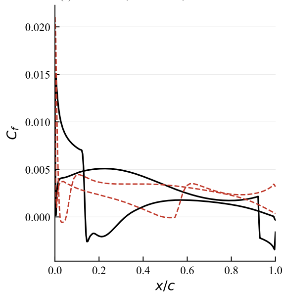
(c) M = 0.65 , \alpha = 4.5^\circ , Re = 1.8 \times 10^6
