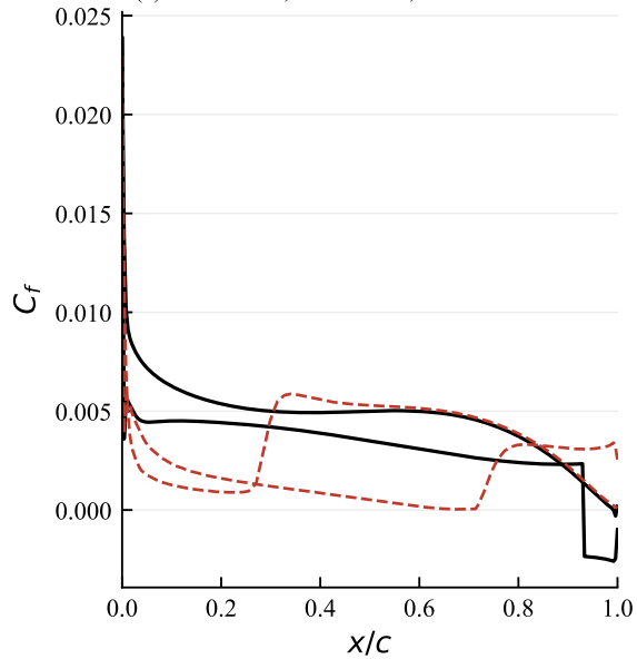
(a) M = 0.30 , \alpha = 2.1^\circ , Re = 1.7 \times 10^6
