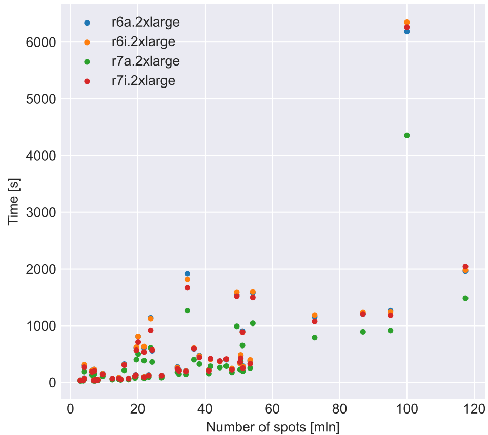
STAR execution times for different instance types
