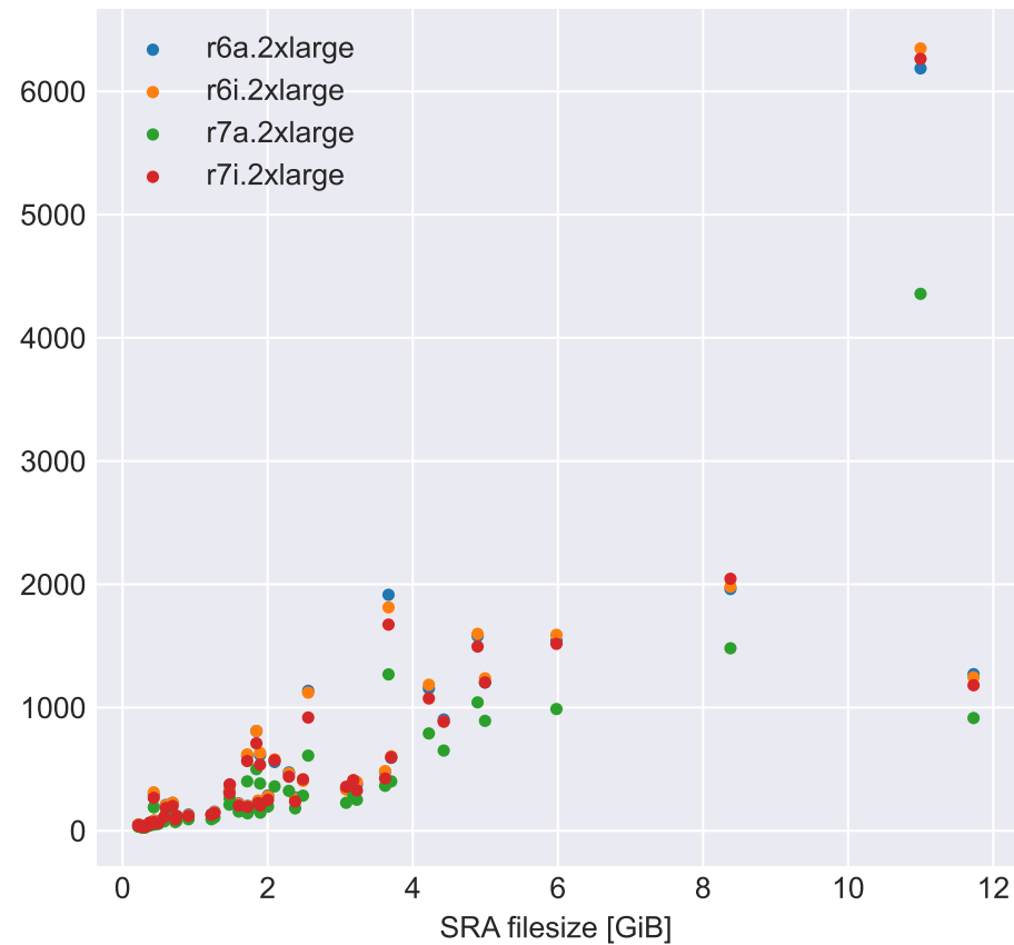
STAR execution times for different instance types
