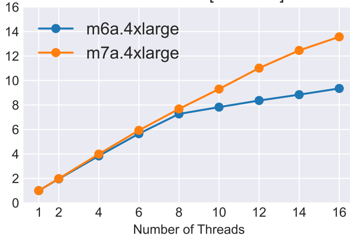
SRR20688788 [2.02 GiB]
