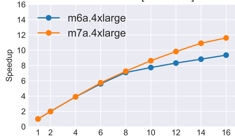
SRR11869226 [10.28 GiB]
