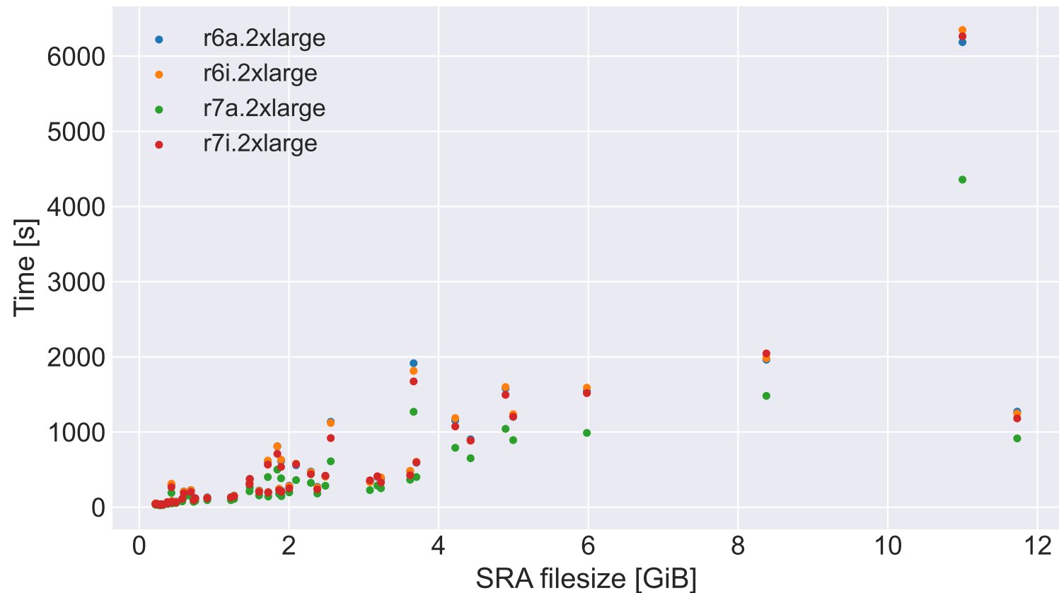
STAR execution times for different instance types
