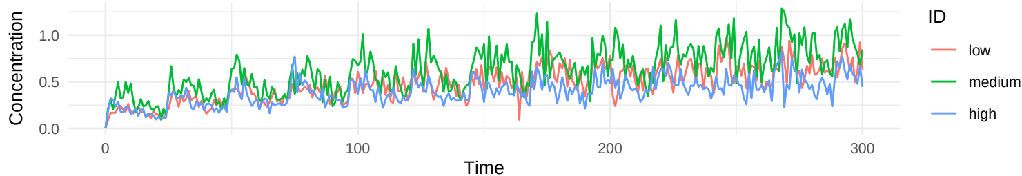
Scenario: strm_2 statm_2 covm_12 clint_pooled covs_unchanged
