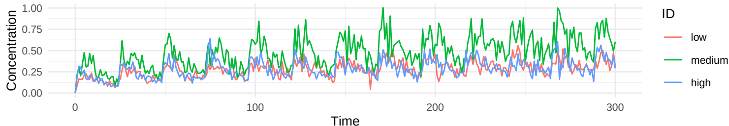
Scenario: strm 2 statm 2 covm 17 clint pooled covs unchanged
