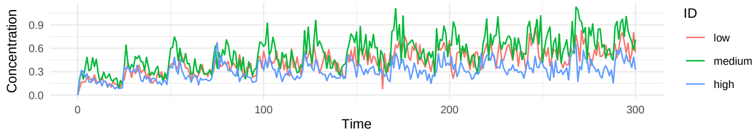
Scenario: strm 2 statm 2 covm 13 clint pooled covs unchanged
