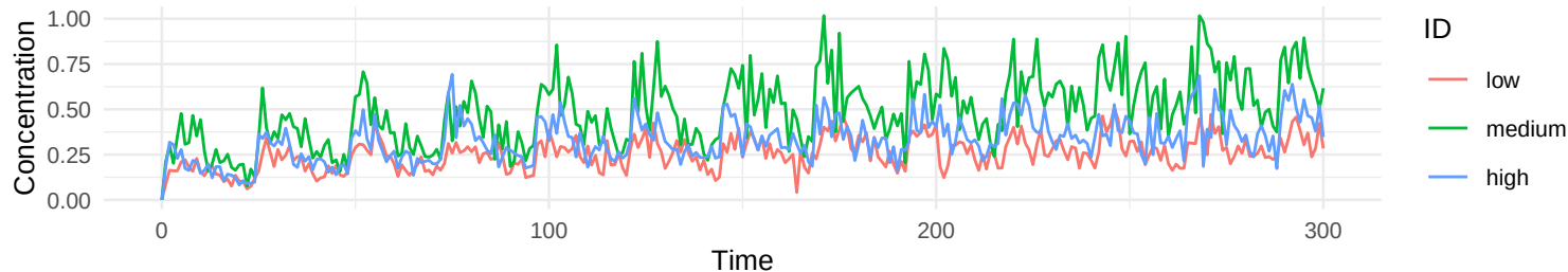
Scenario: strm_2 statm_2 covm_15 clint_pooled covs_unchanged
