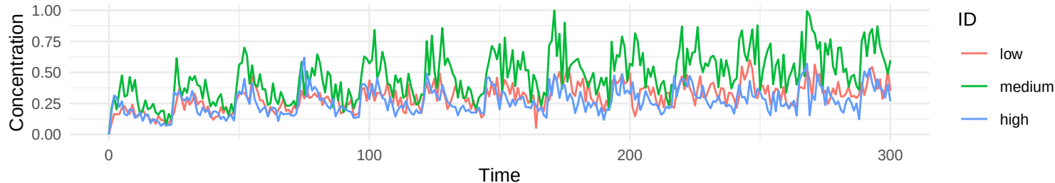
Scenario: strm 2 statm 2 covm 16 clint pooled covs unchanged
