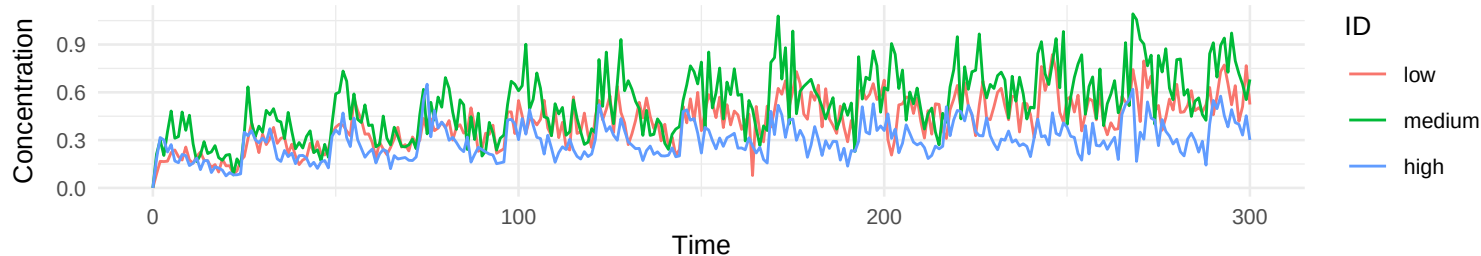
Scenario: strm 2 statm 2 covm 14 clint pooled covs unchanged
