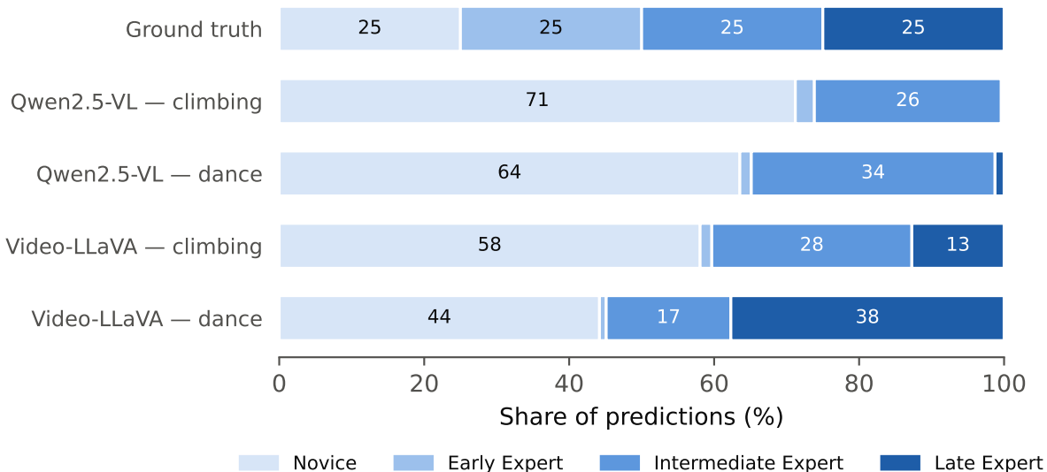
Four-class prompts: predictions collapse onto 1-2 labels
