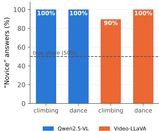
Binary prompts: (almost) everyone is a novice
