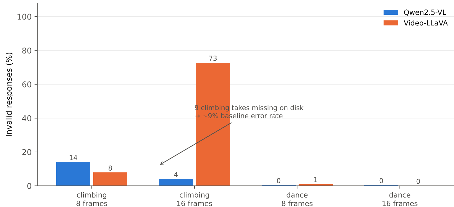
Unusable responses (runtime errors, empty or unclassifiable output)
