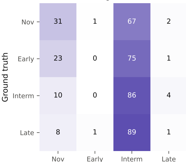
Climbing — Gemini
