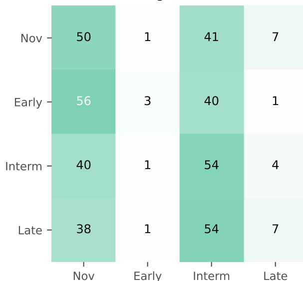
Climbing — Qwen3-VL
