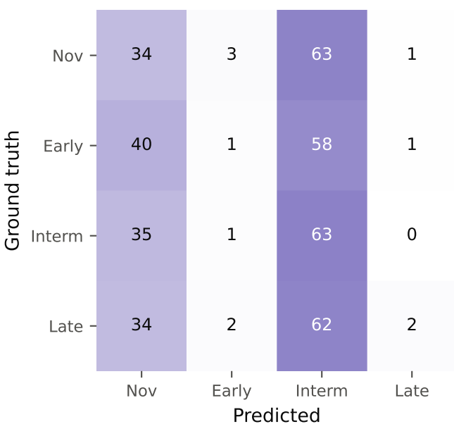
Dance — Gemini
