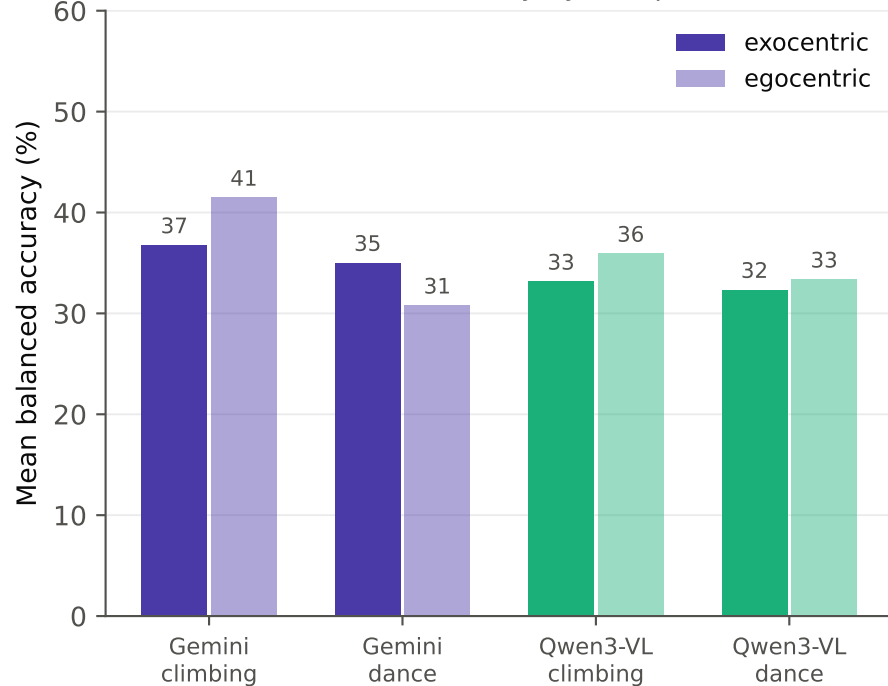
Balanced accuracy by viewpoint
