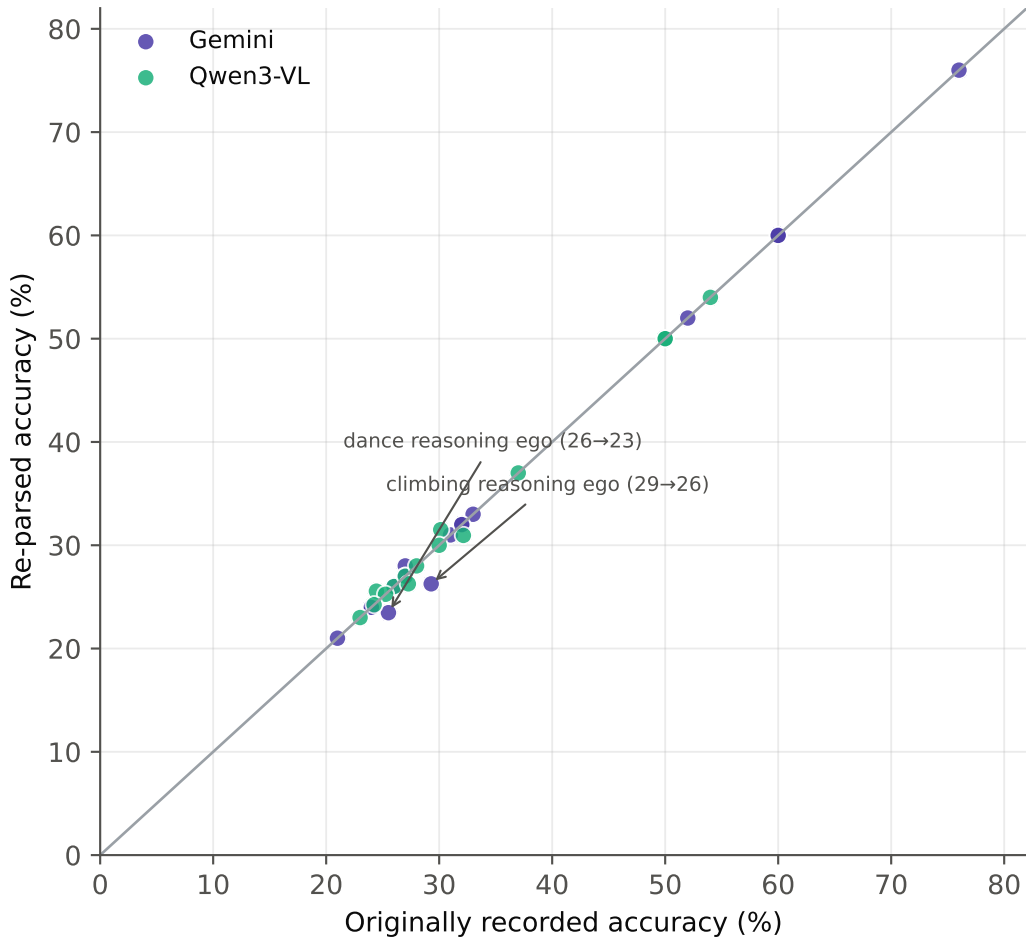
Effect of re-parsing model answers
