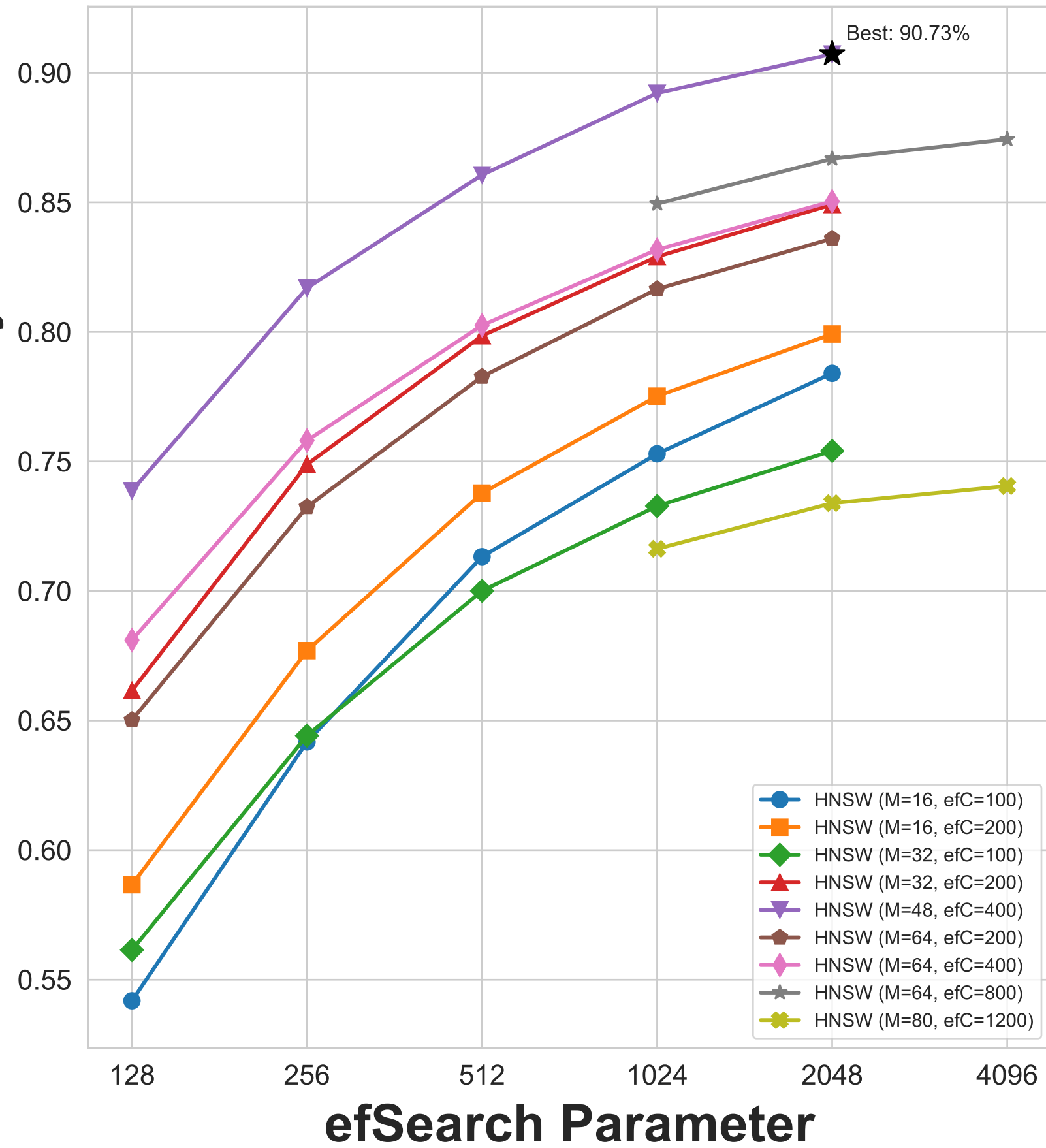
(a) HNSW
