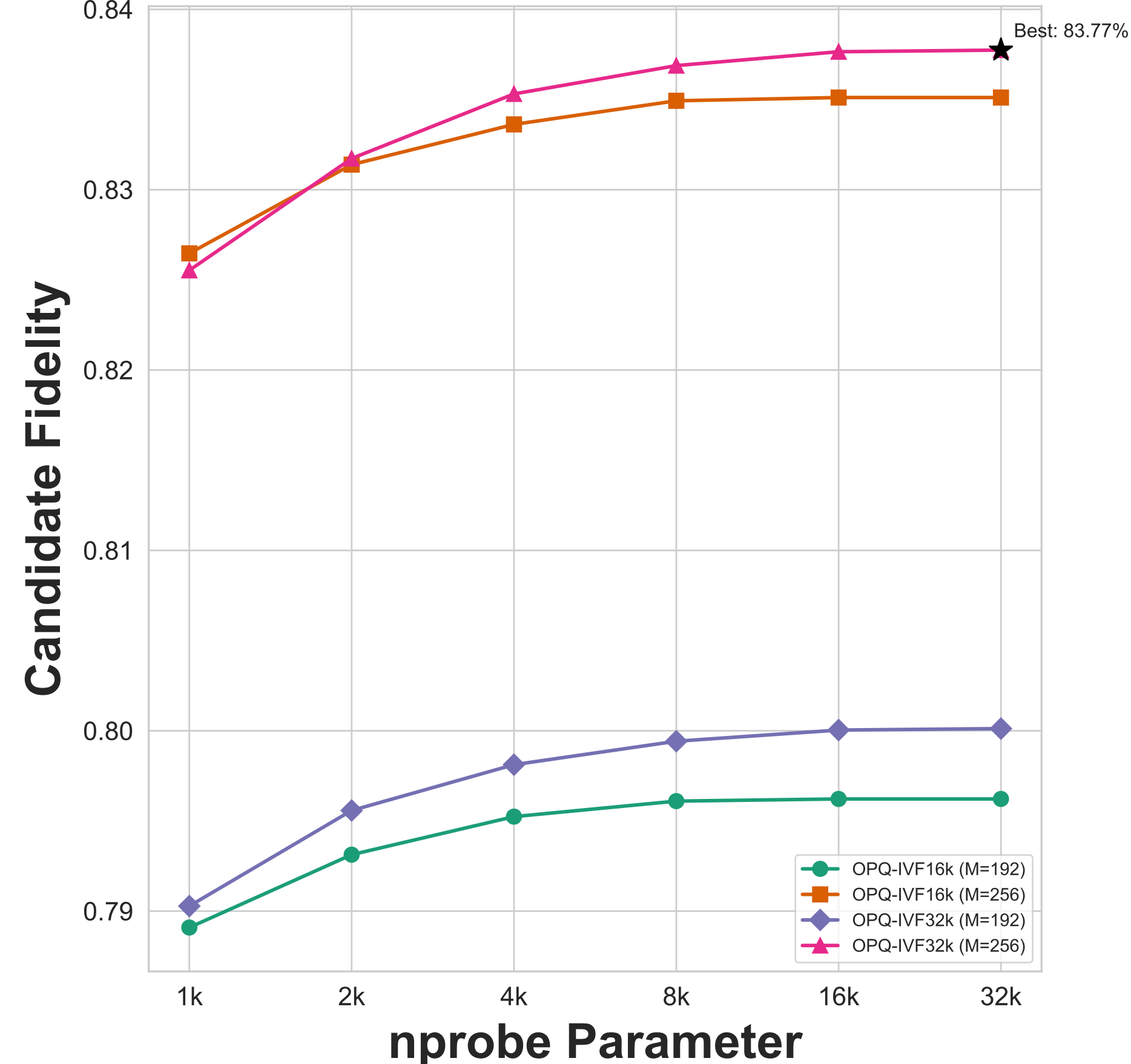
(c) O-IVFPQ
