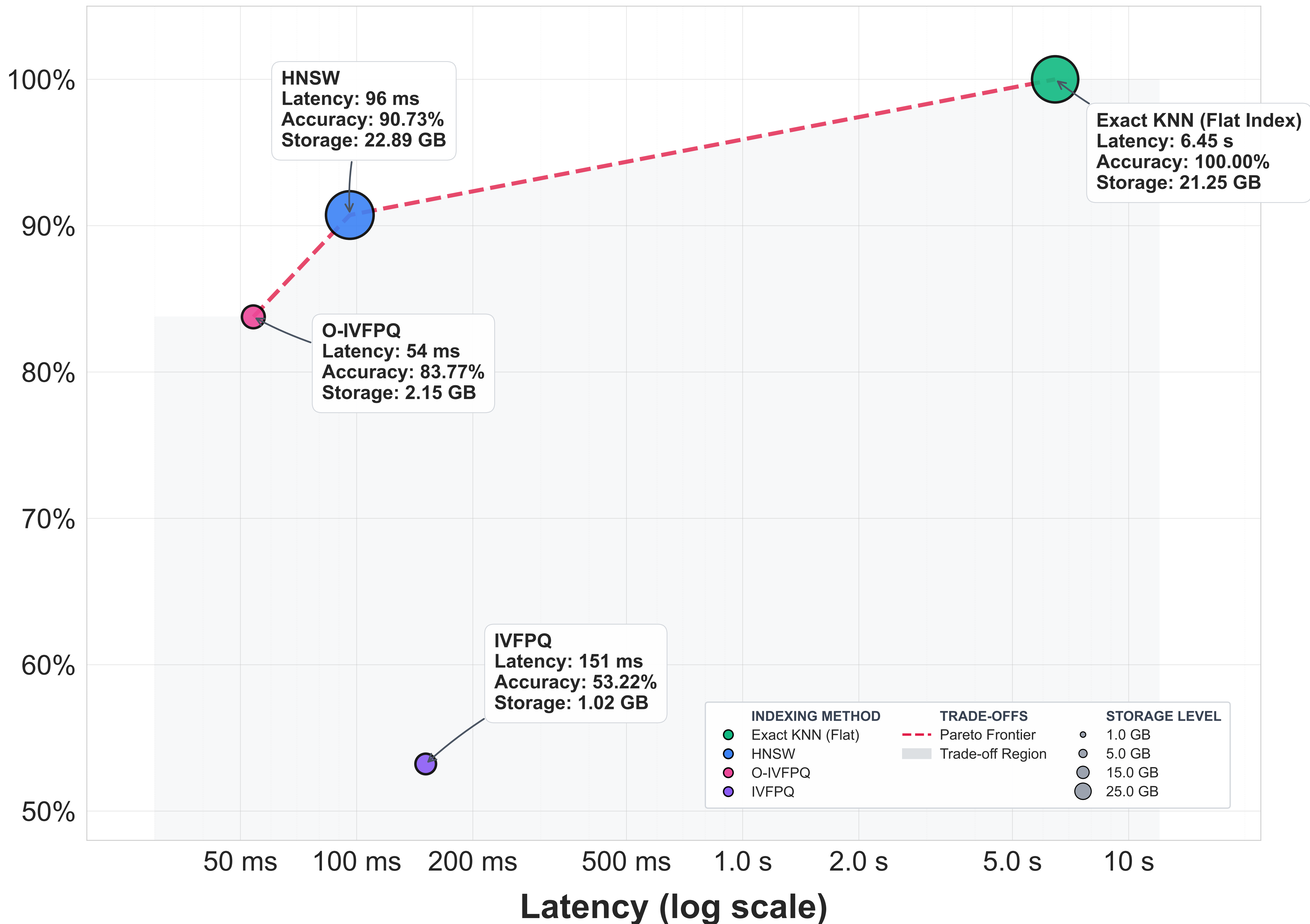
Candidate Fidelity (Acc vs KNN %)
