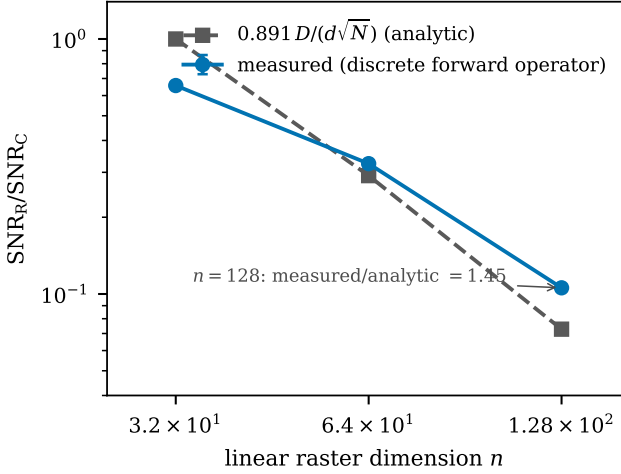
Figure 2: Validation of the discrete operator: measured deconvolution noise penalty vs. the analytic estimate of Toth & Turyshv (2021). The \sim 45\% difference at n = 128 reflects discrete pixel-averaging of the central singularity and finite-domain boundary attenuation.
