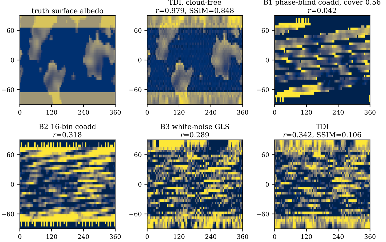
Figure 3: Reconstruction gallery for the fiducial 87.33-day campaign ( n = 64 , M_p = 16 , t_s = 1800 s, 16-node exposure quadrature ). Top: truth surface albedo; TDI reconstruction of the rotating cloud-free planet ( r = 0.979 , \text{SSIM} = 0.848 ); phase-blind coadd (B1) at realized cover 0.56, which is essentially featureless ( r = 0.042 ). Bottom, all at realized cover \simeq 0.56 : 16-bin phase-binned coadd (B2), white-noise GLS (B3), and TDI. The gross continental dichotomy is recovered, but fine features are erased by weather.
