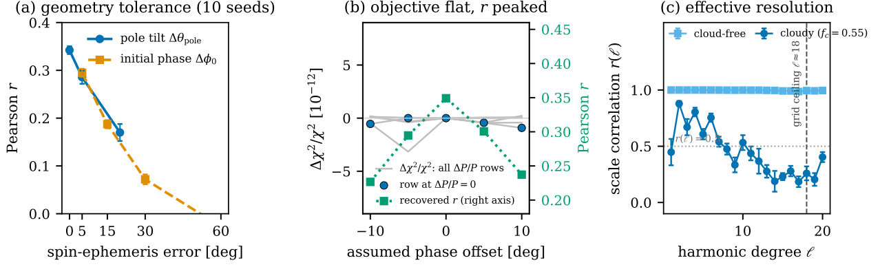
Figure 6: Robustness suite. (a) Correlation vs. spin-pole tilt and assumed initial-phase error (10 paired seeds; the zero-error point is the fiducial fit). (b) Whitened \chi^2 , re-referenced to its own value at zero phase, as a function of assumed phase offset for every trial period on the grid: the relative variation is \leq 10^{-11} , i.e. the objective is exactly flat in phase, while the reconstruction quality r (right axis, green) peaks at the truth — the phase error is observable through image quality, not through the likelihood (Section 5.9). (c) Scale-dependent correlation r(\ell) for the cloud-free and cloudy campaigns (10 seeds, \pm 1 SE), with the \ell \leq 20 grid ceiling marked.
