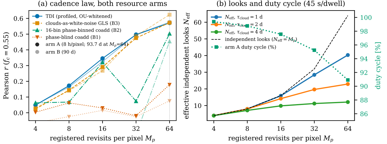
Figure 5: Cadence law under the two resource ledgers , all values read directly from the shipped archives. (a) Pearson r vs. registered revisits M_p for the profiled TDI, the white-noise GLS and the two coadd baselines; solid lines are arm A ( M_{pt_s} = 8 h, 6 paired seeds) and faded lines arm B (89.87 d wall clock). The trend is monotone and saturating, and the two arms agree within the paired standard error at every M_p . (b) The quantity that actually saturates: the effective independent look count N_{\text{eff}} at \tau_{\text{cloud}} = 1, 2, 4 d against the N_{\text{eff}} = M_p line of perfectly decorrelated weather (Table 8), with the arm-A duty cycle under the 45 s/dwell overhead ledger on the right axis.
