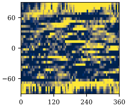
B3 white-noise GLS, f_c=0.55 r=0.29
