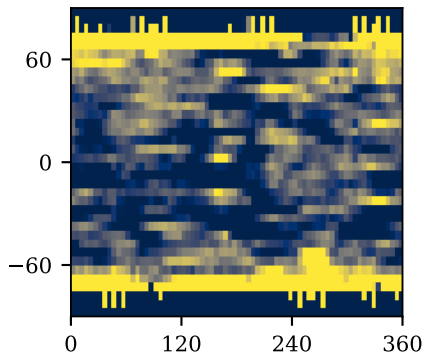
B2 phase-binned, f_c=0.55 r=0.13
