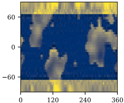
TDI, cloud-free r=0.99 , SSIM=0.92
