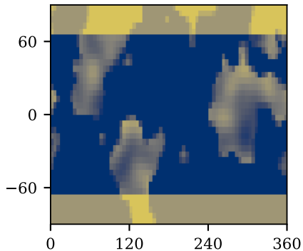
truth surface albedo
