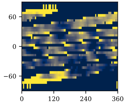
TDI r=0.342 , SSIM=0.106
