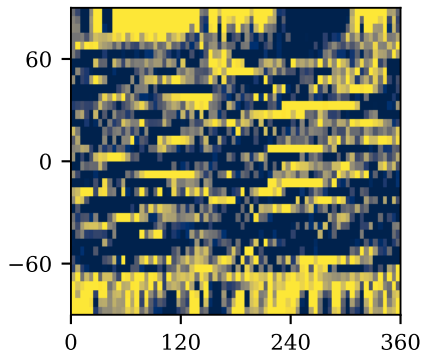
B3 white-noise GLS r=0.289
