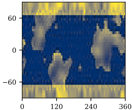
B3 white-noise GLS r=0.289
