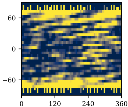
B2 16-bin coadd r=0.318
