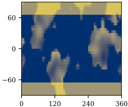
B2 16-bin coadd r=0.318
