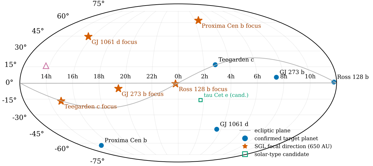
Figure 8: Celestial placement (equatorial Mollweide) of the five confirmed targets (blue circles), candidate \tau Cet e (green square), and their SGL focal directions (orange stars, purple triangle). The gray line marks the ecliptic plane. Ross 128 and Teegarden c focal lines lie in the ecliptic ( \beta_{\text{ecl}} \approx 0^\circ ), minimizing departure \Delta\nu .
