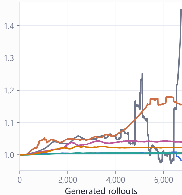
Actor perplexity
