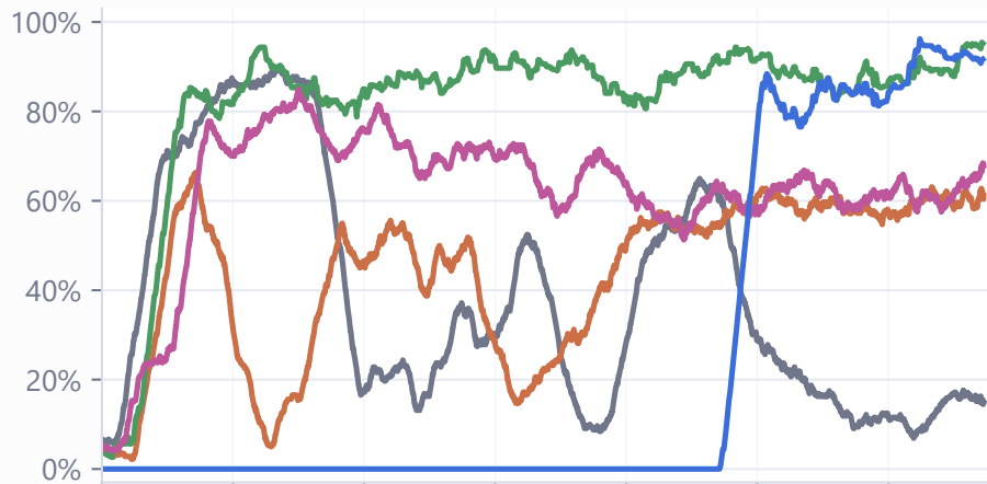
Format accuracy
