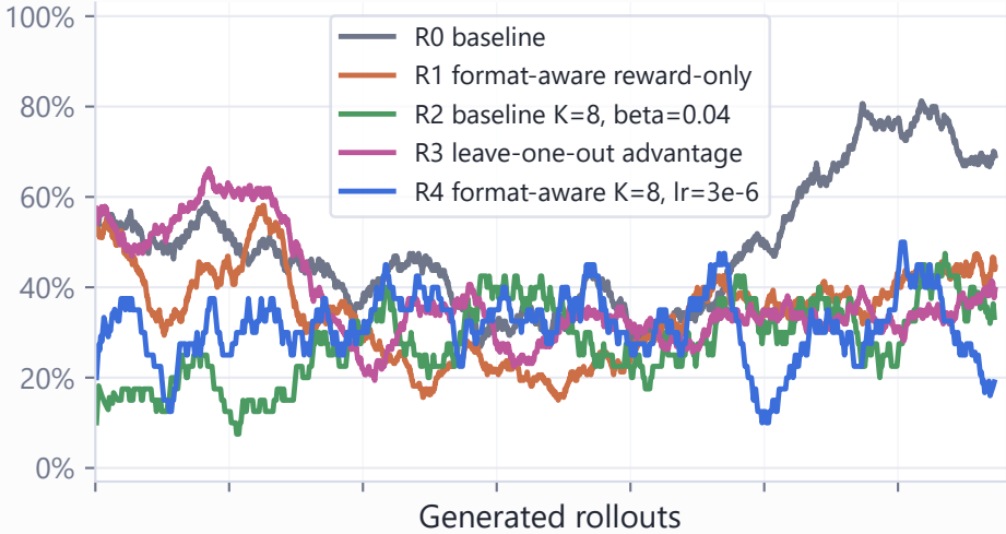
Zero-reward-std groups
