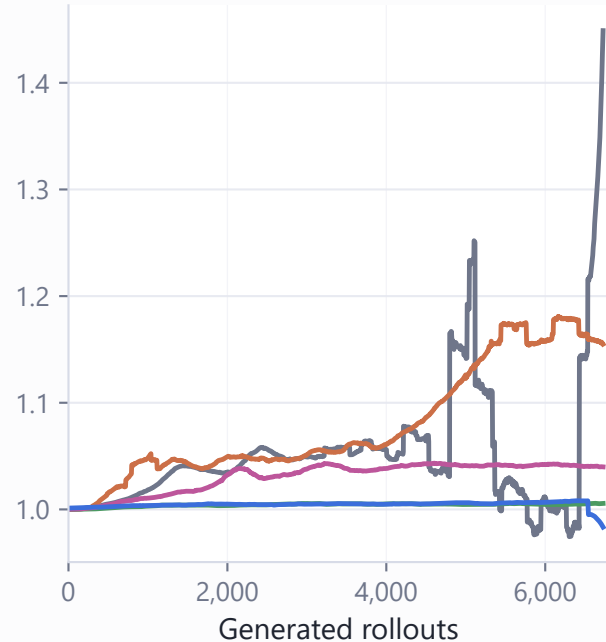
Actor perplexity
