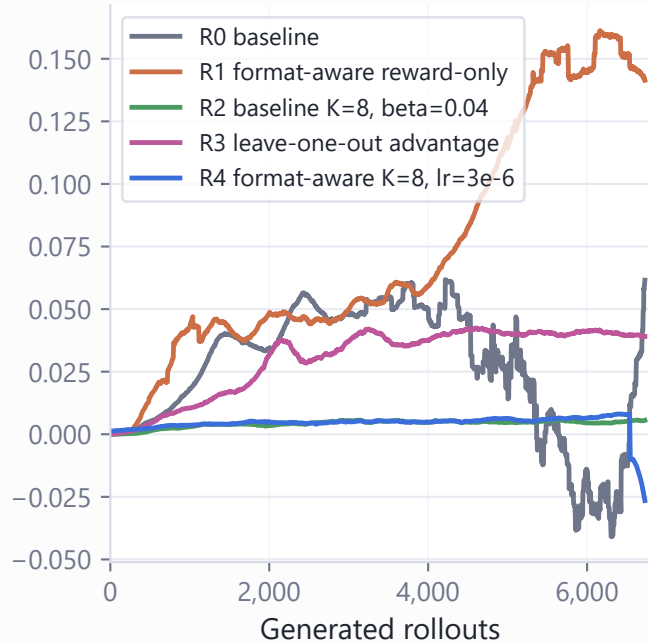
Loss
