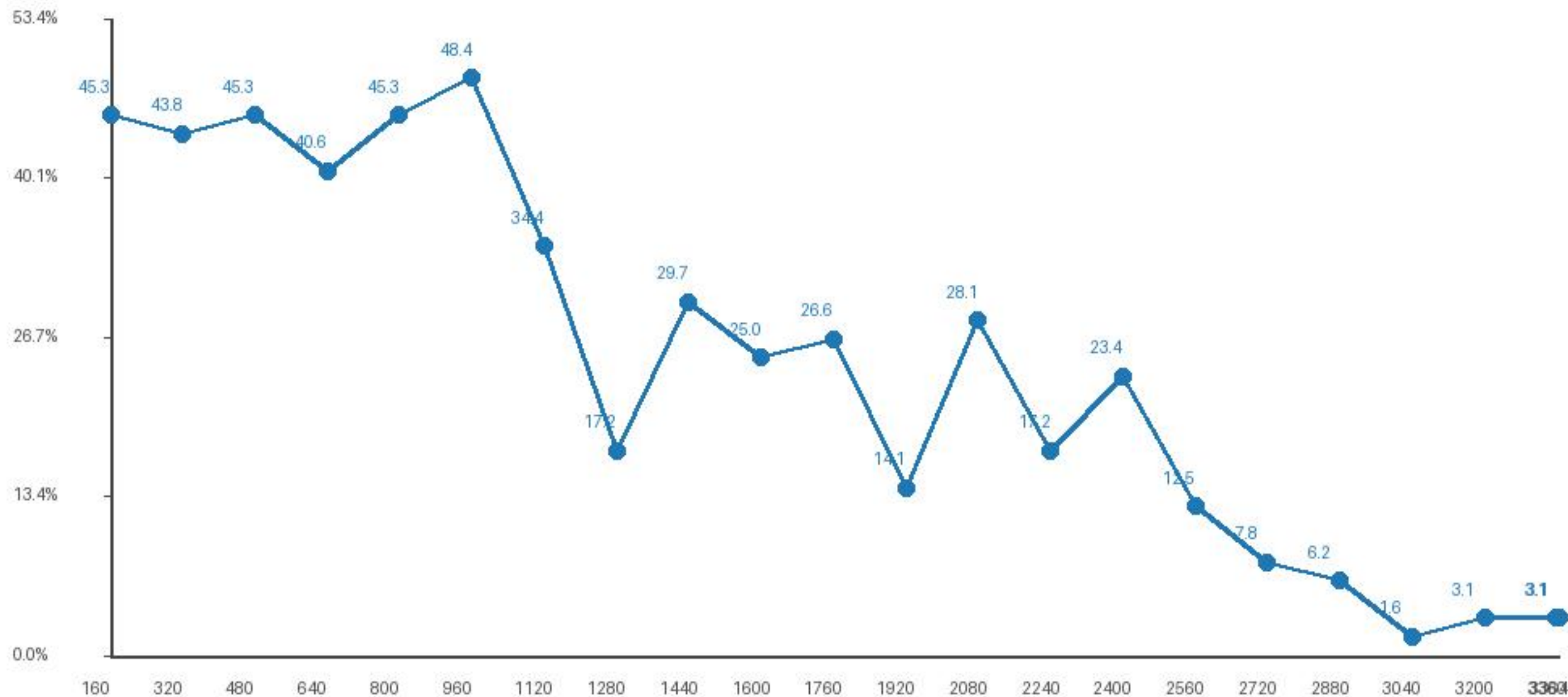
Checkpoint GSM8K accuracy
