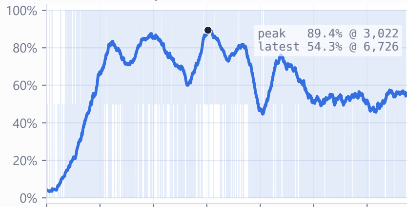
Format accuracy
