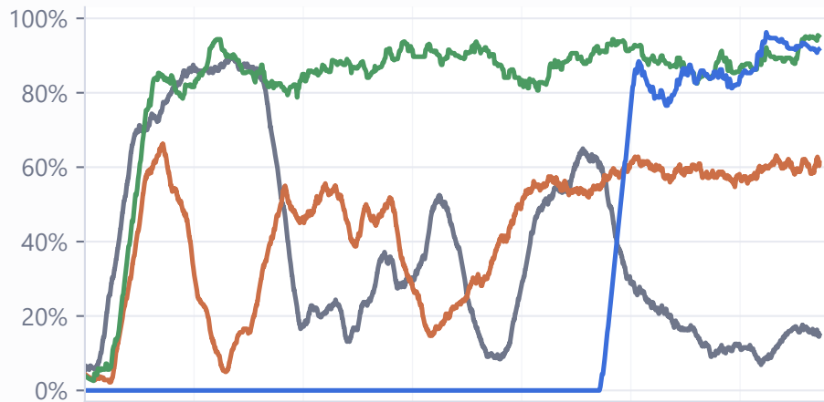
Format accuracy
