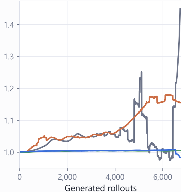
Actor perplexity
