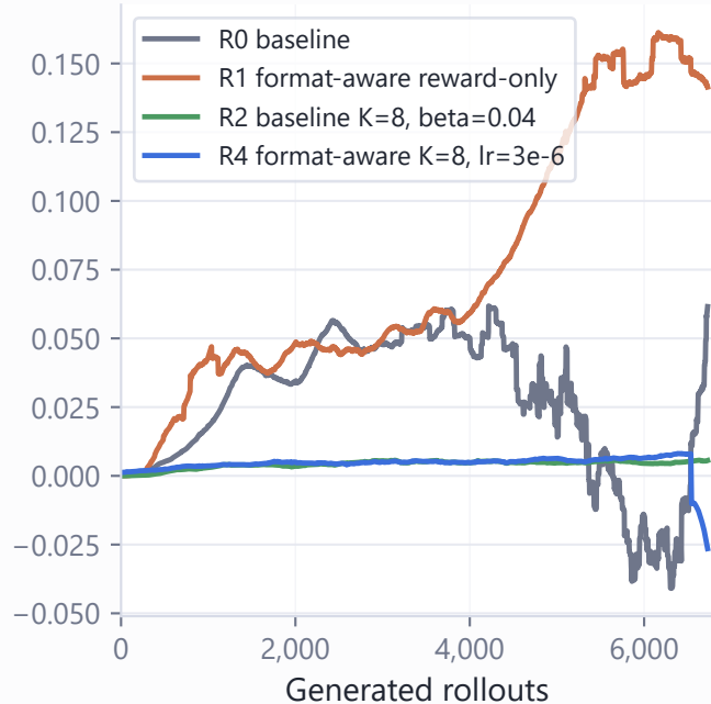
Loss
