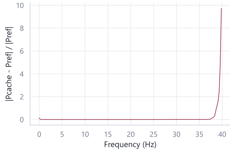
Passband error, PSD RMSE=0.0050
