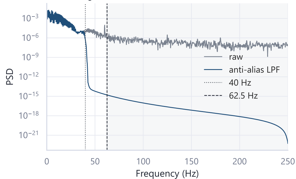
Anti-aliasing PSD
