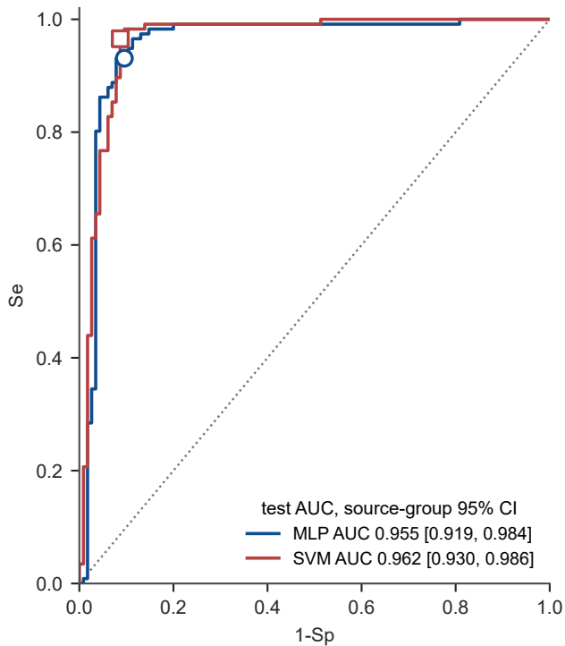
a held-out test ROC
