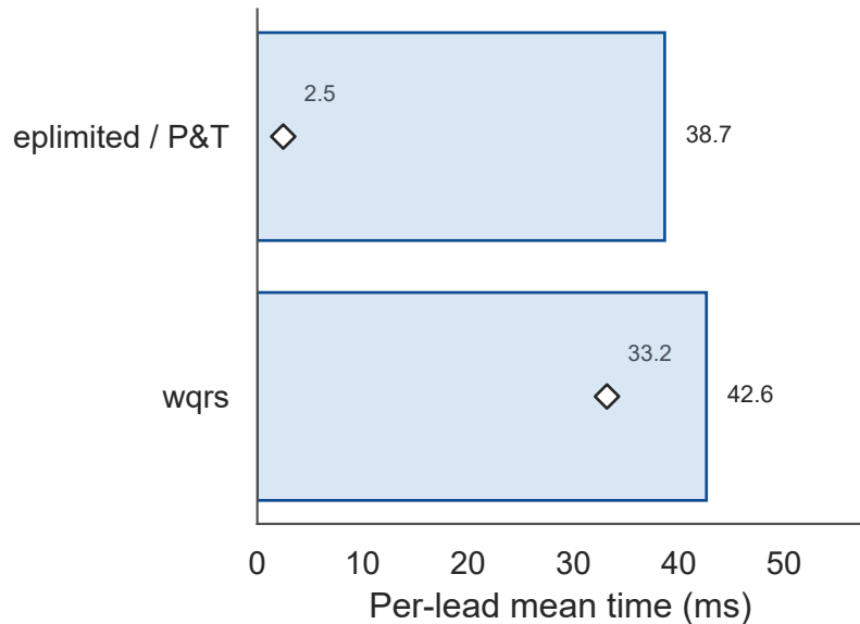
a detector comparison ■ this run ◇ paper Table 8
