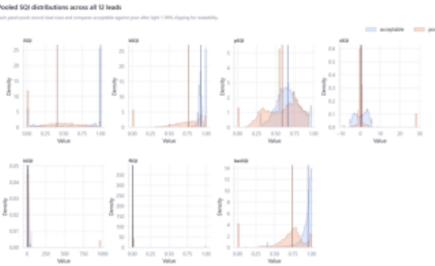
04_pooled_sqi_distributions
