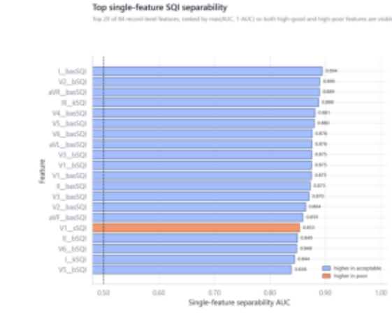
13_single_feature_auc_top20
