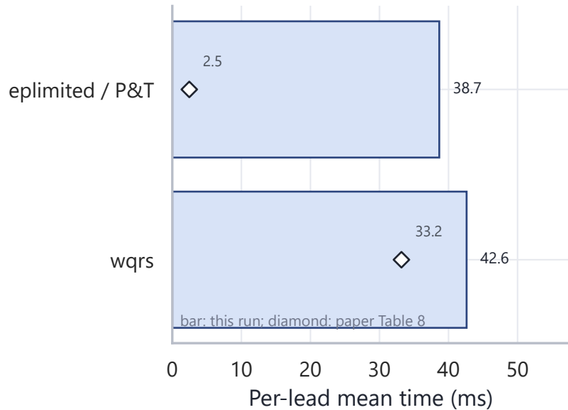
detector comparison
