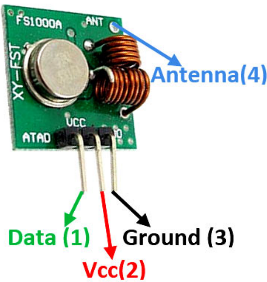
(/sites/default/files/component_pin/433-MHz-RF-Transmitter-Module-Pinout_0.jpg)
