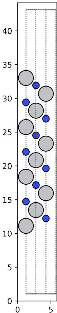
Relaxed Ti-terminated TiN(111) slab — side view
