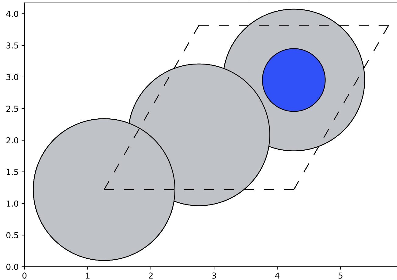
TiN(111) surface — top view
