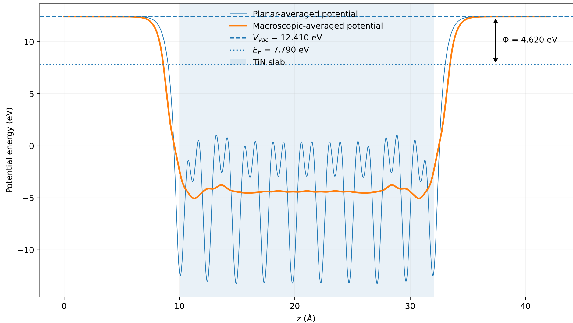
Ti-terminated TiN(111): vacuum work function
