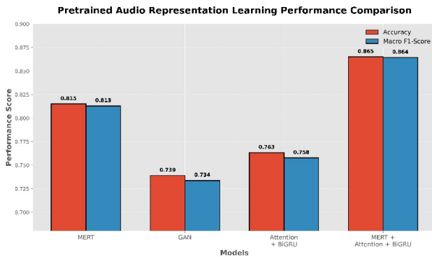
Fig. 3: Comparative Performance Analysis of Accuracy and F1-Score for Pretrained Audio Representation Learning Models
