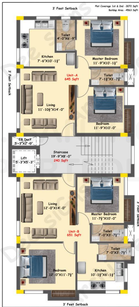
FIRST &amp; SECOND FLOOR
