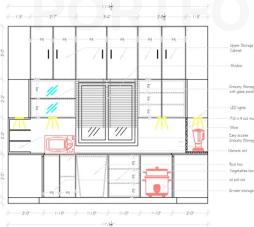
B-side
