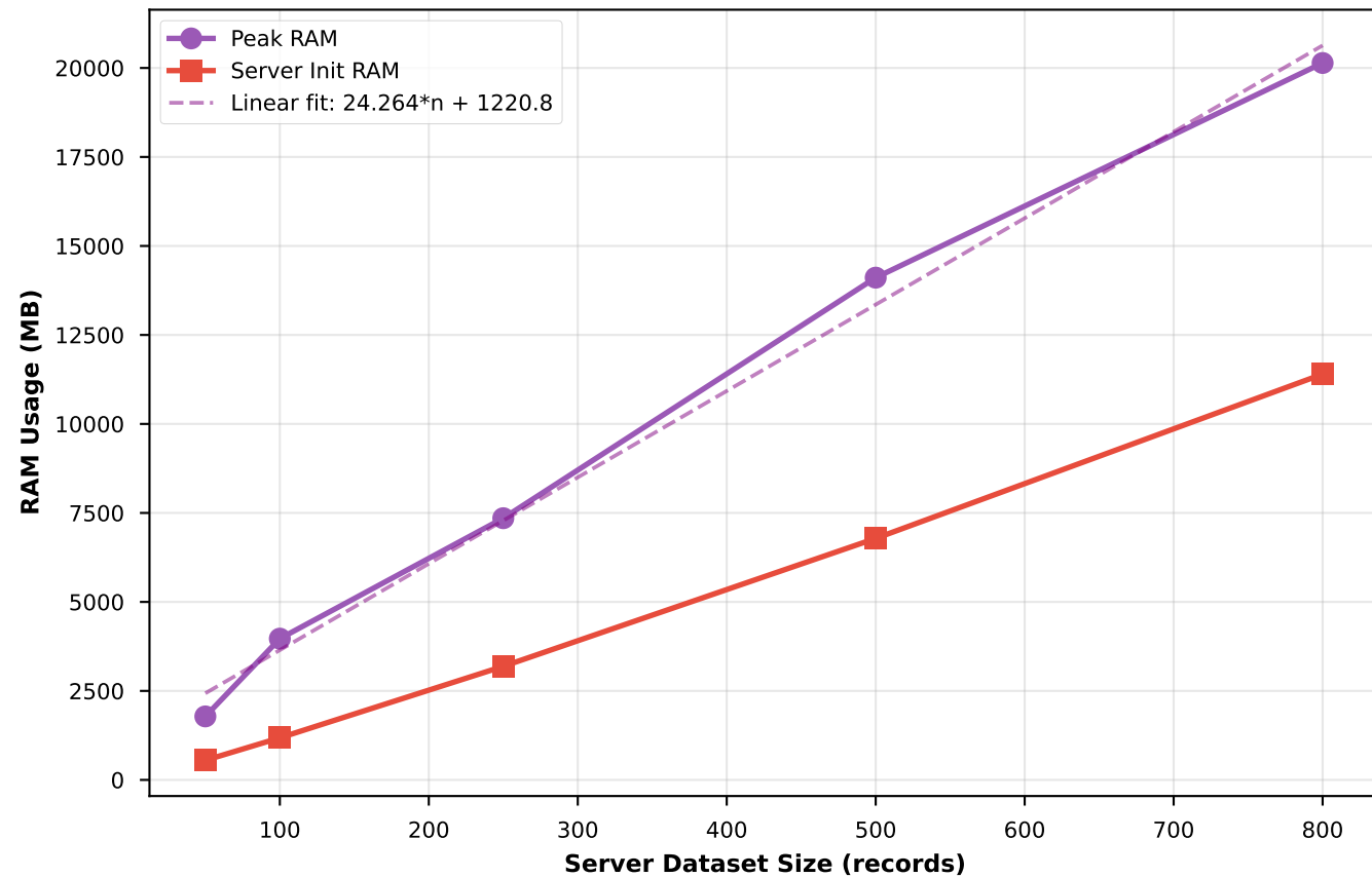
RAM Consumption vs Dataset Size
