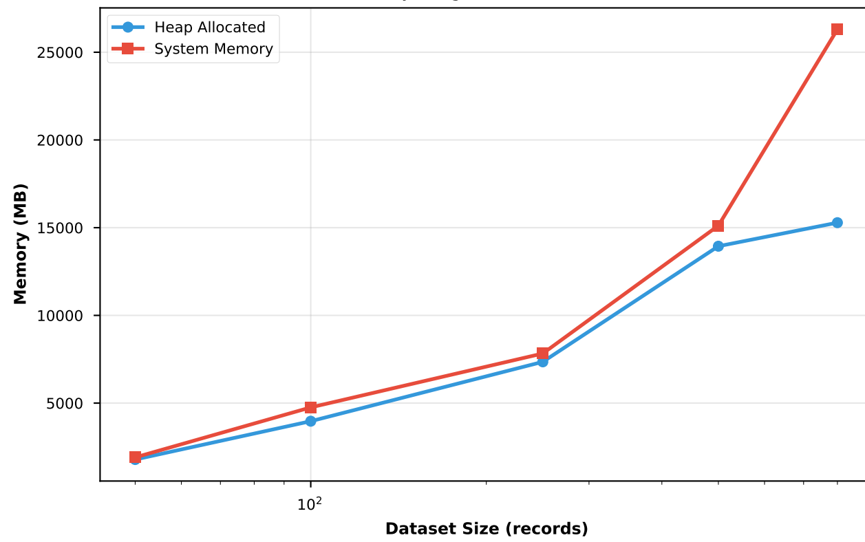
Go Memory Usage Across Dataset Sizes
