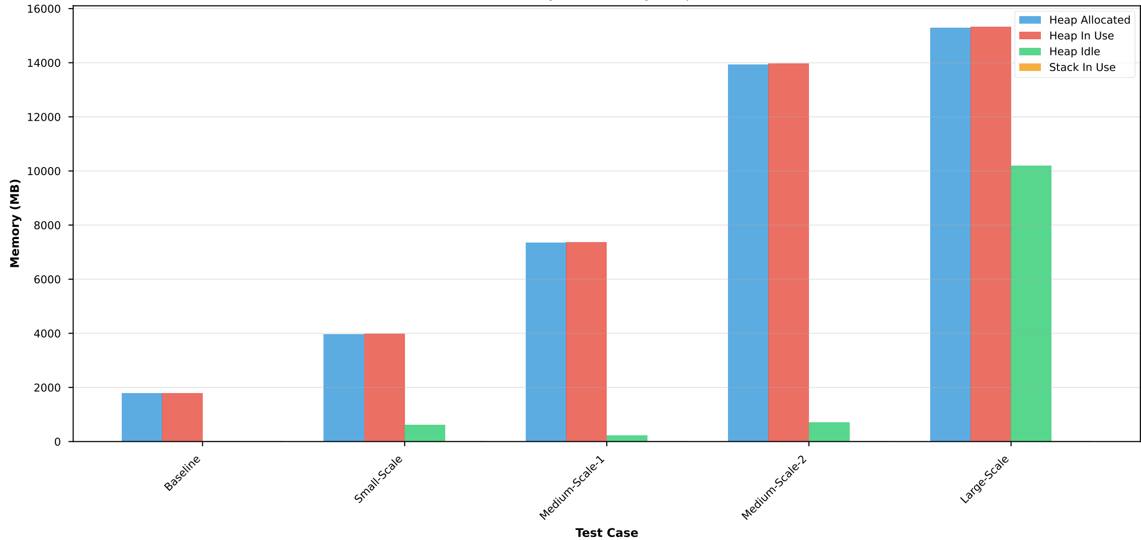
Go Memory Breakdown by Component
