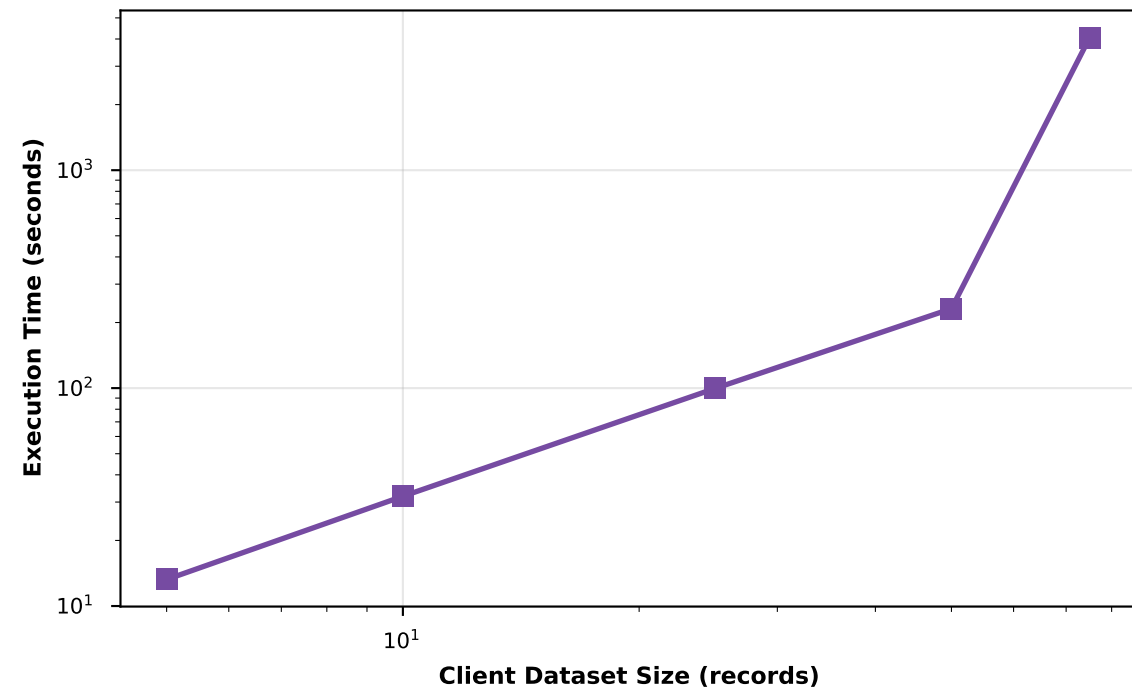
Client Dataset Size vs Execution Time
