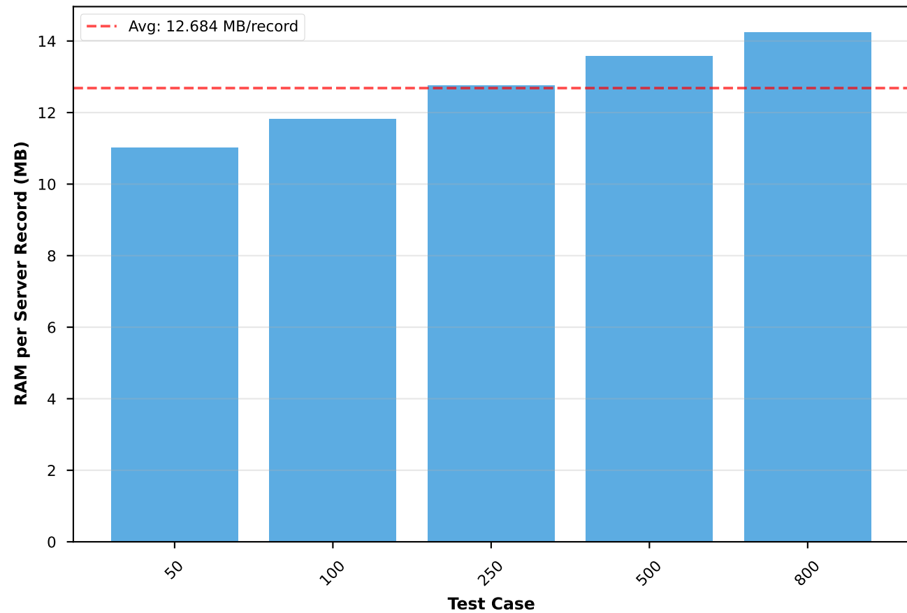
Memory Efficiency: RAM per Record
