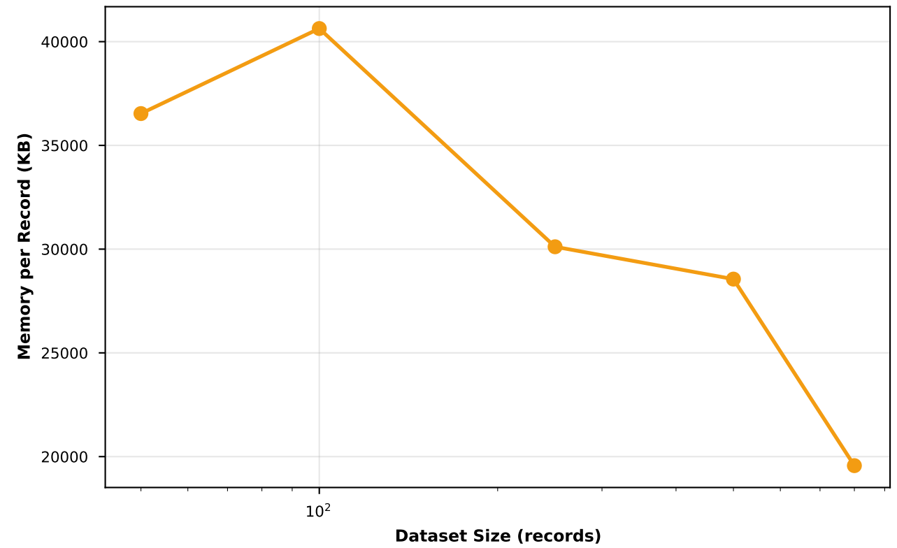
Memory Efficiency - Heap per Record
