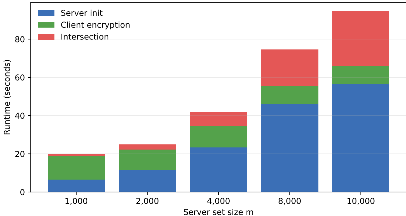
LE-PSI single-node runtime breakdown
