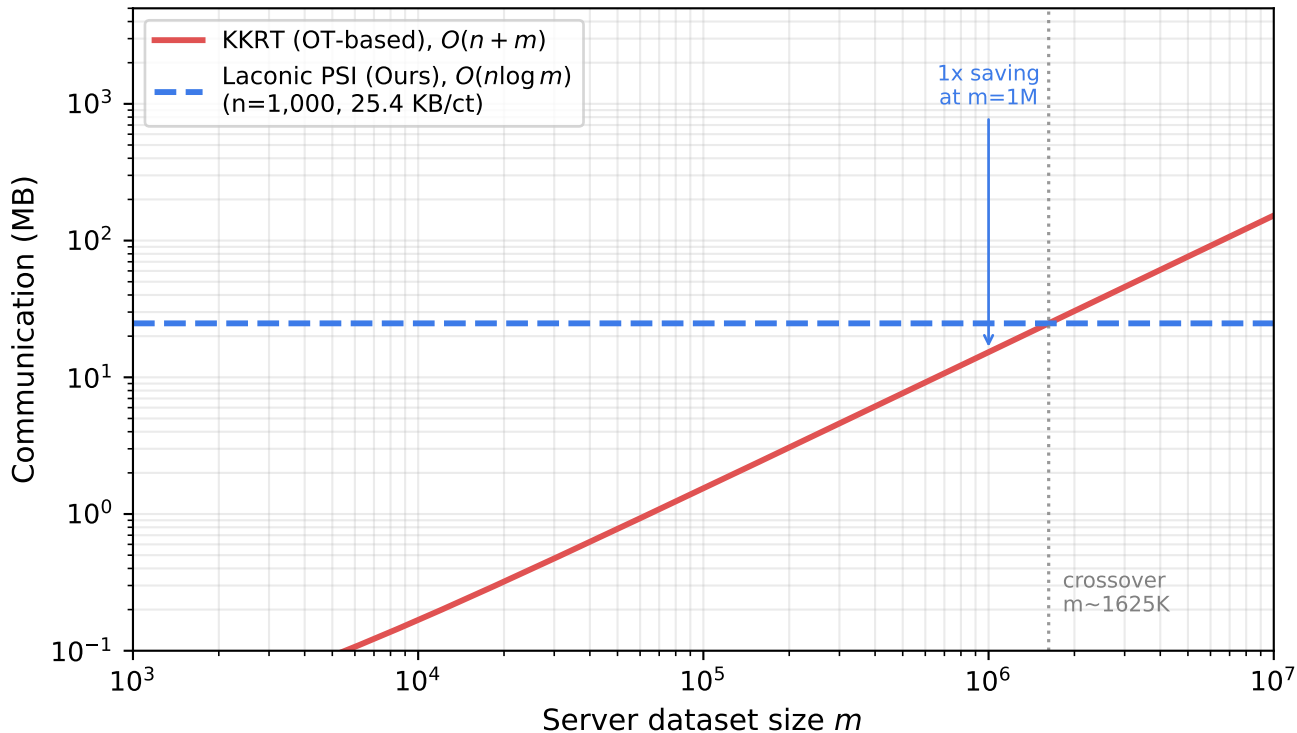
Communication Scaling: Laconic PSI vs KKRT ( n=1,000 client records, 25.4 KB per ciphertext)
