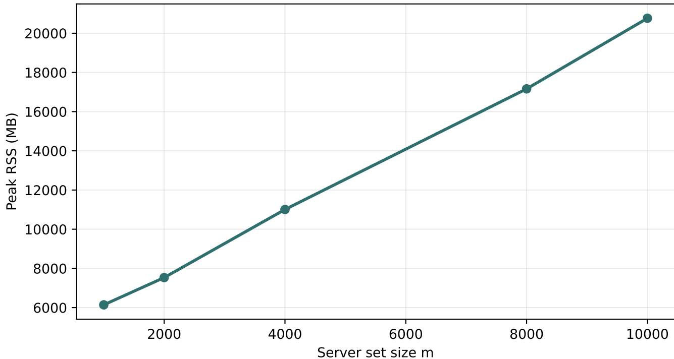
LE-PSI single-node peak RSS
