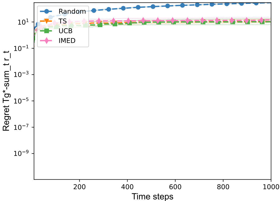
MAB-Bernoulli-v0
