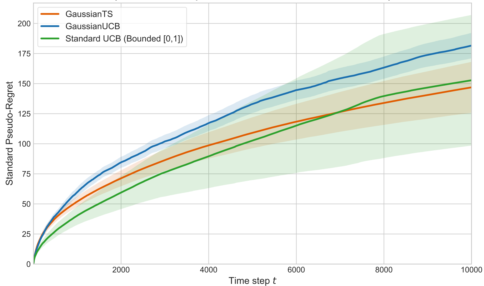
Gaussian Bandit: GaussianTS vs GaussianUCB vs Standard UCB (Evaluation of exploration bounds under Gaussian noise)
