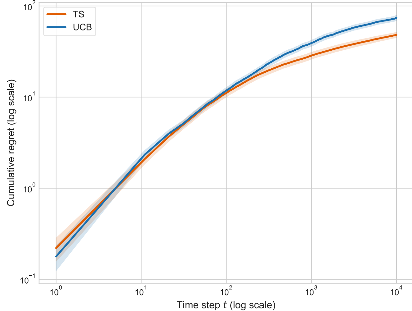
Practitioner Regret ( \epsilon^*=0.0500 )
