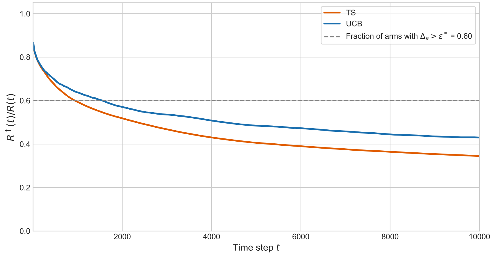
Ratio of Practitioner Regret to Standard Regret
