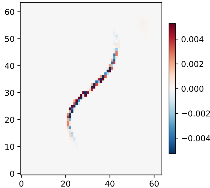
Shape Error
