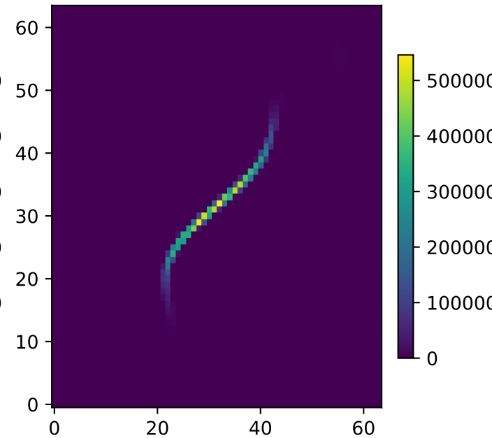
Physical Pred
