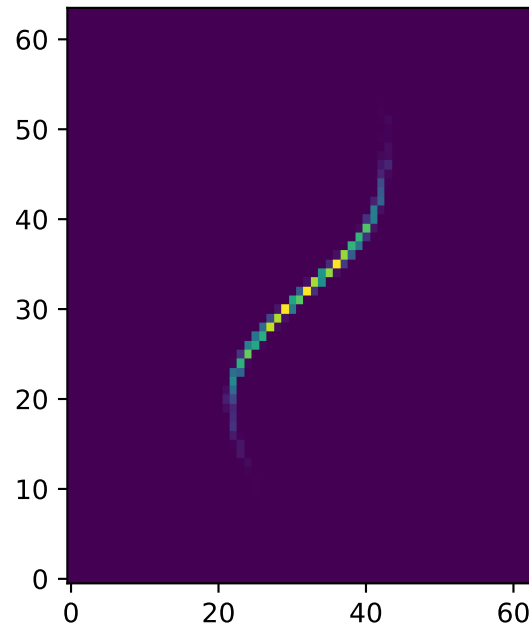
Physical Truth
