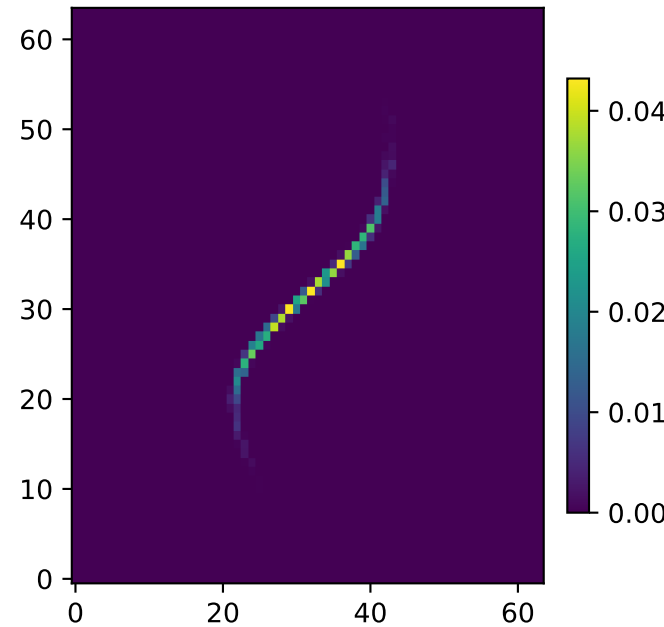
Ground Truth
