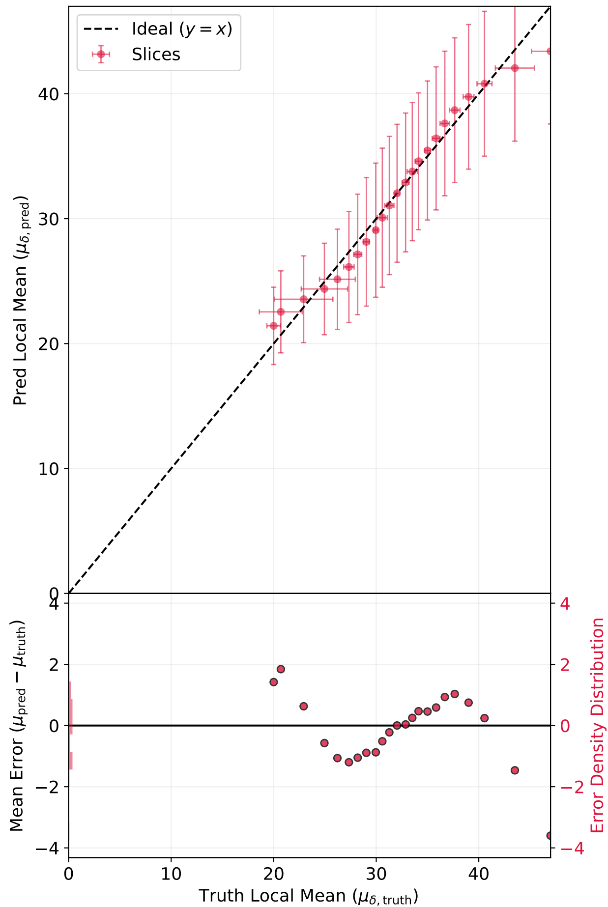
Constant-z Slices ( \delta Distribution Means)
